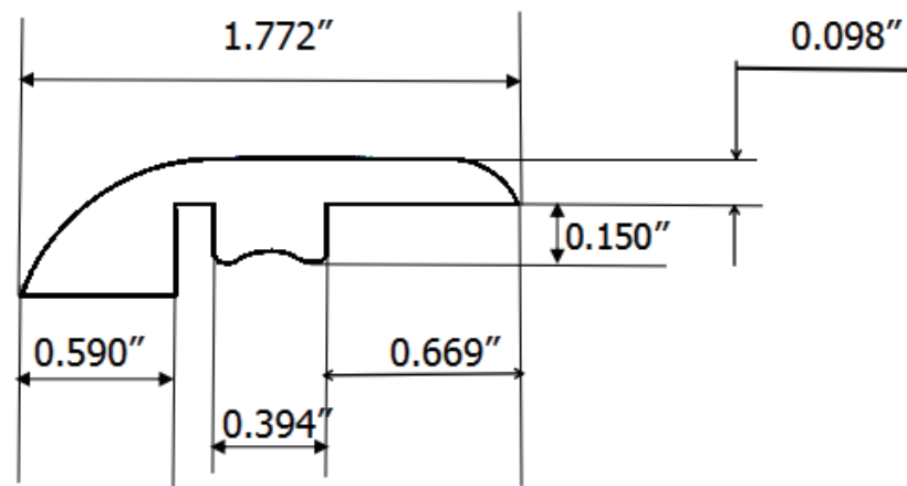
Reducer
