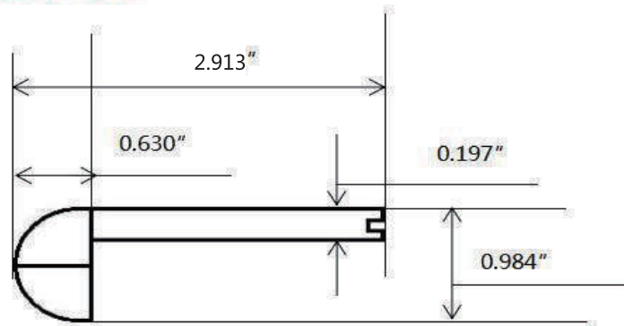
Flush Stair Nose:
